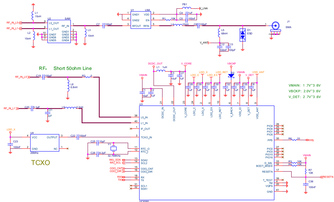
Figure 1-2 Reference design of DCDC mode
